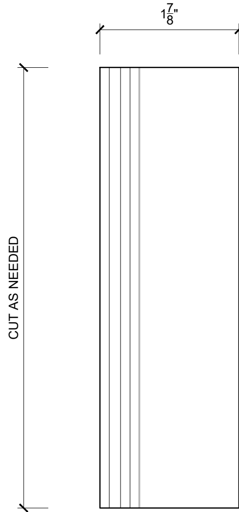
2 PL5 (RECEIVER) - FRONT PL5-A SCALE 9"=1'-0"
