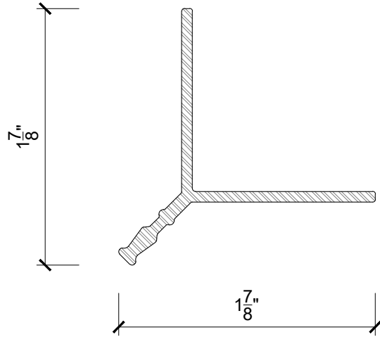
1 PL5 (RECEIVER) - PROFILE PL5-A SCALE 1'-0"=1'-0"
