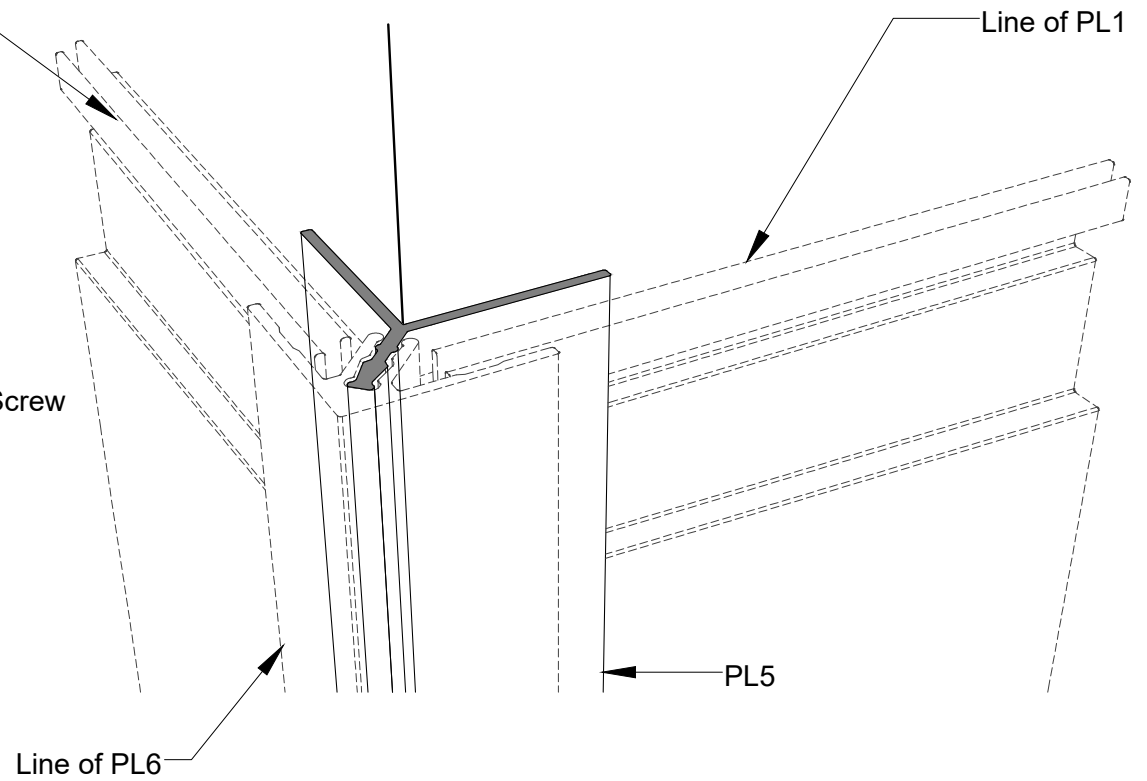
2 PL5 (RECEIVER) - APPLICATION - 3D VIEW PL5-B SCALE NTS
