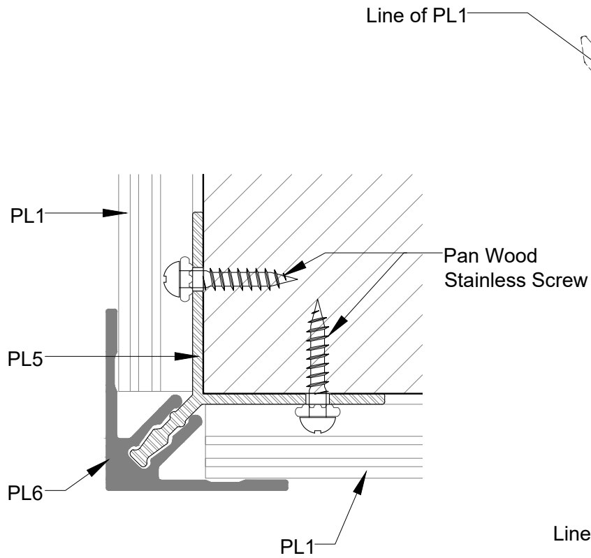
1 PL5 (RECEIVER) - APPLICATION PL5-B SCALE 1'-0"=1'-0"
