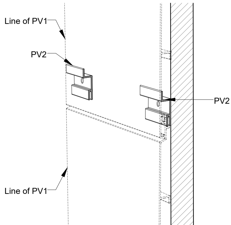
2 PV2 - APPLICATION - 3D VIEW PV2-B SCALE NTS
