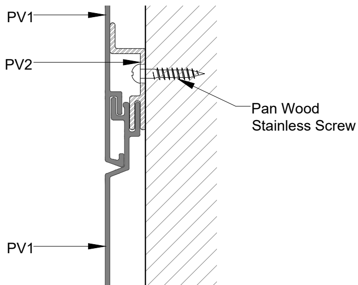
1 PV2 - APPLICATION PV2-B SCALE 9"=1'-0"
