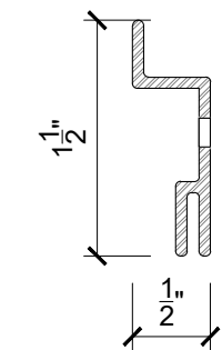
1 PV2 - PROFILE PV2-A SCALE 9"=1'-0"
