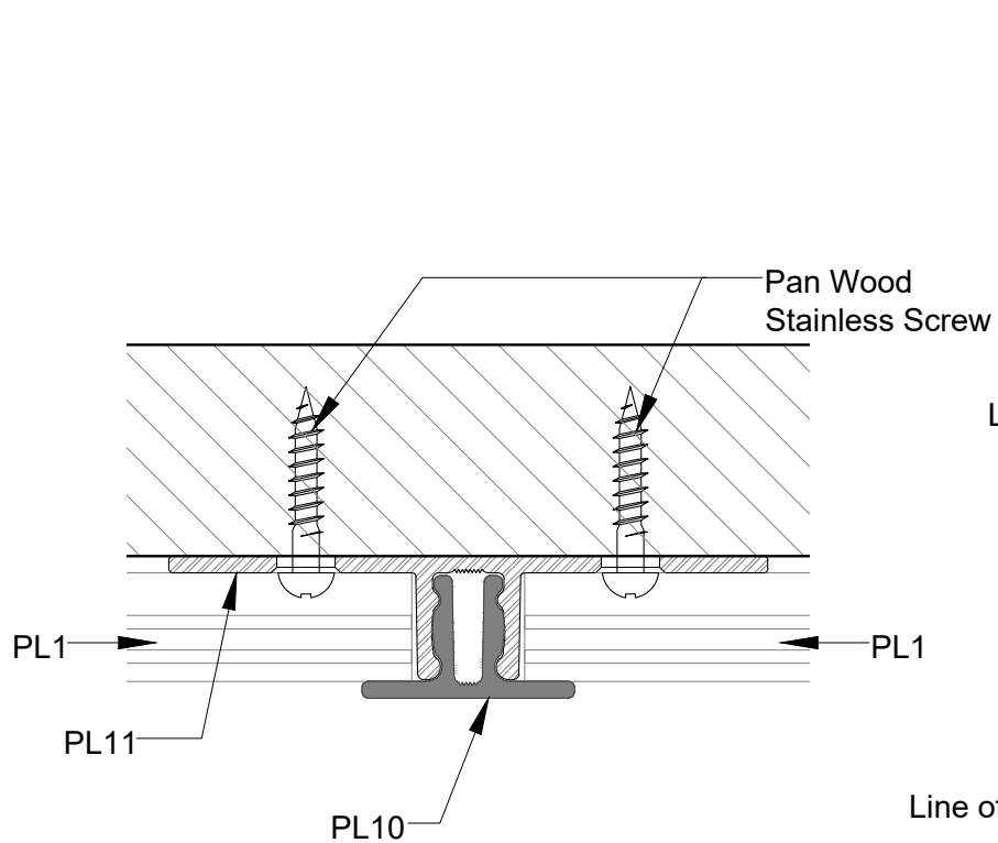
1 PL11 (RECEIVER) - APPLICATION PL11-B SCALE 1'-0"=1'-0"
