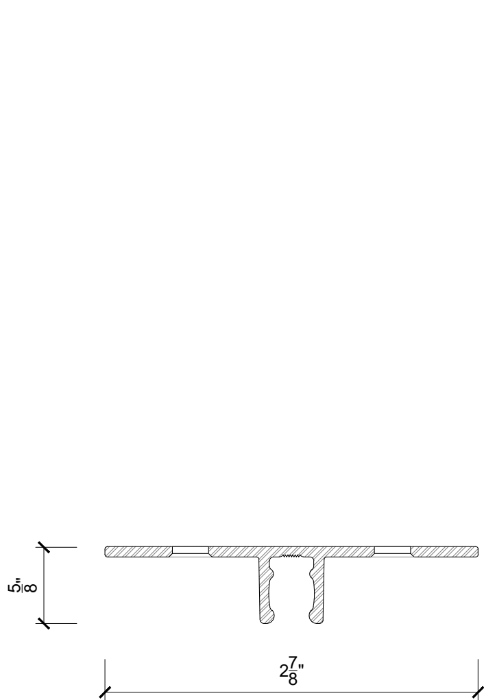
1 PL11 (RECEIVER) - PROFILE PL11-A SCALE 1'-0"=1'-0"
