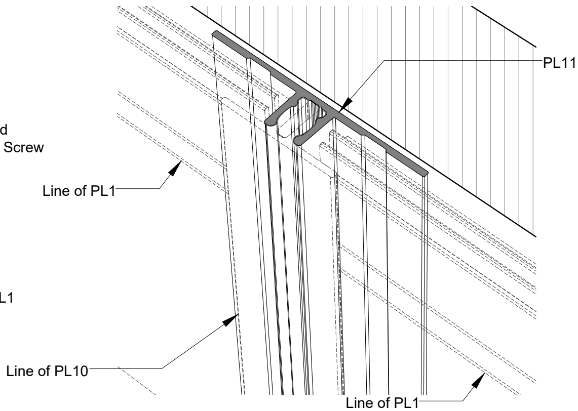
2 PL11 (RECEIVER) - APPLICATION - 3D VIEW PL11-B SCALE NTS
