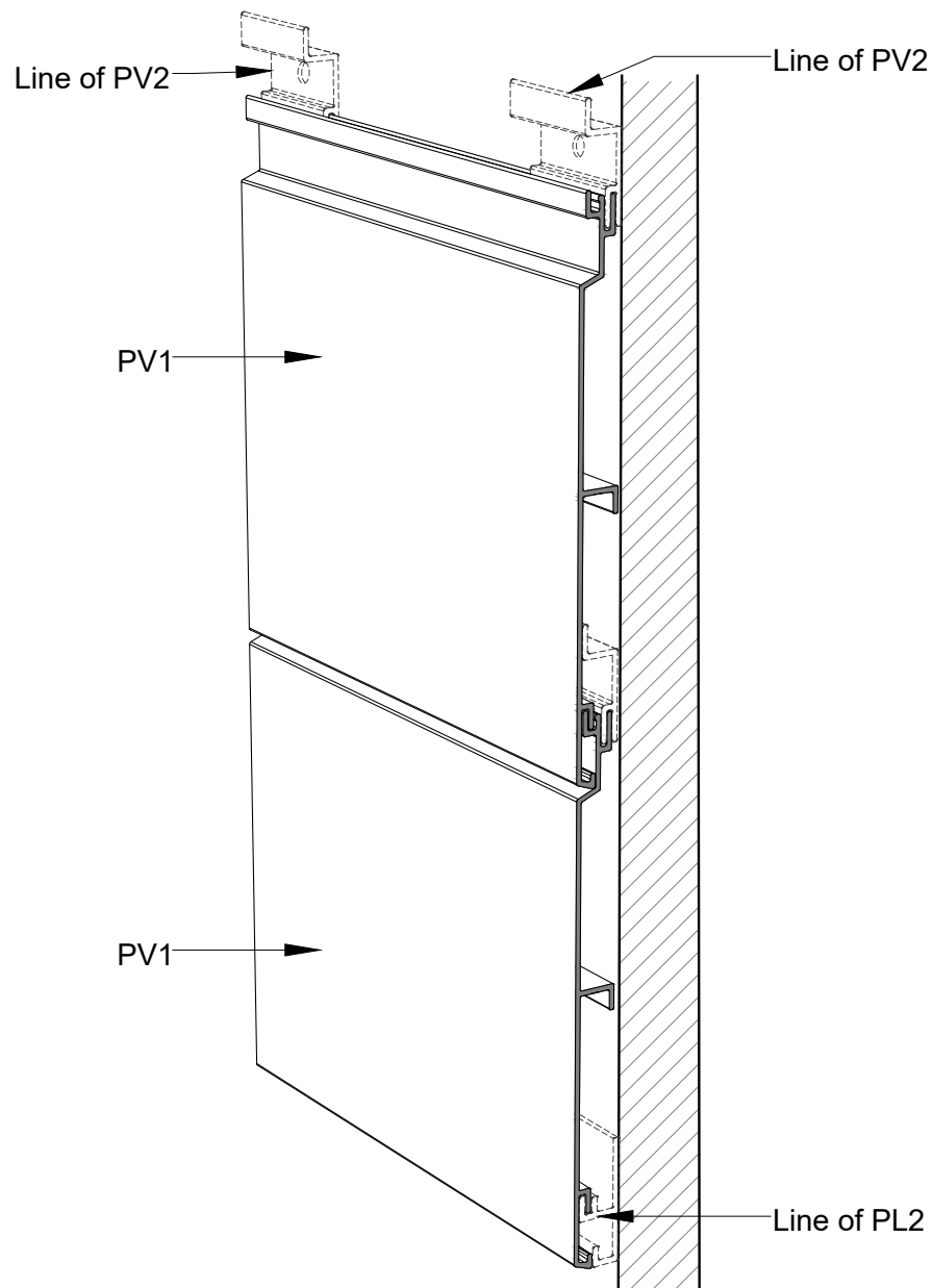
2 PV1 - APPLICATION - 3D VIEW PV1-C SCALE NTS
