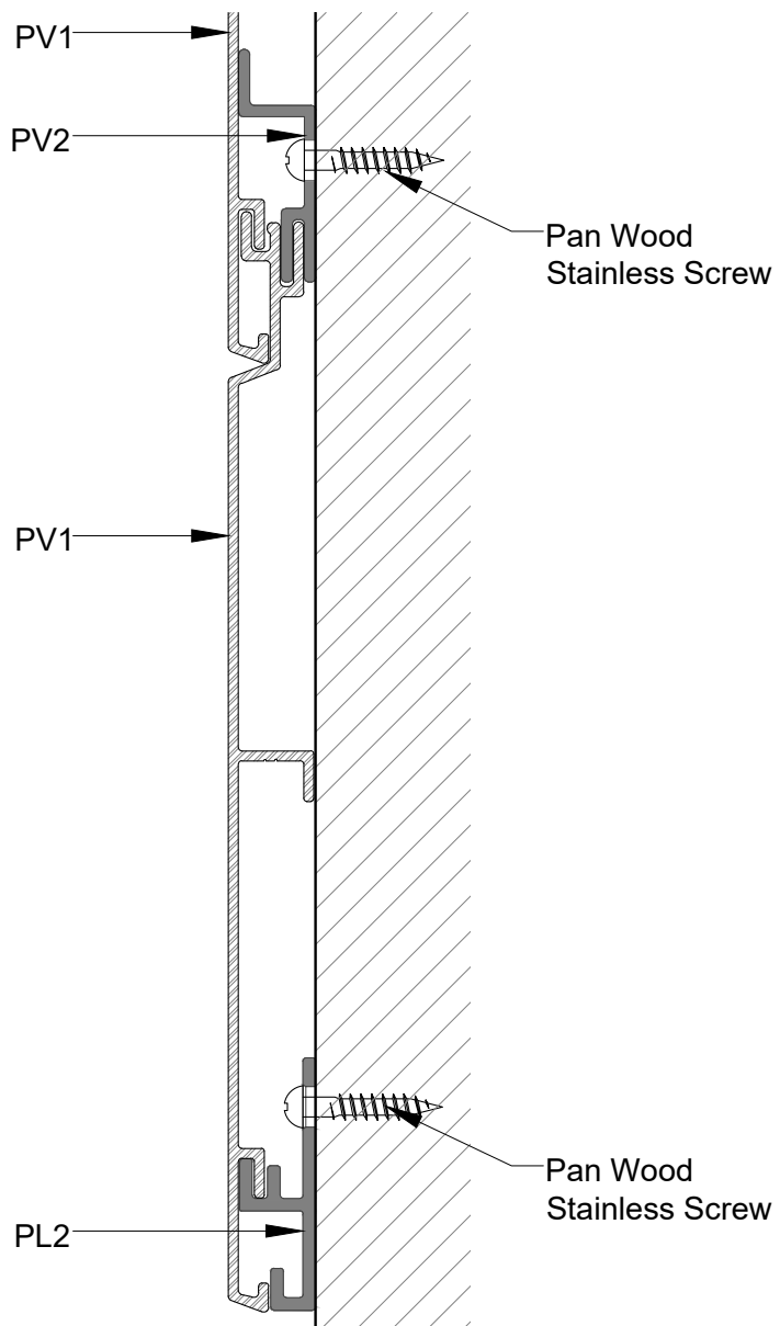
1 PV1 - APPLICATION PV1-C SCALE 9"=1'-0"
