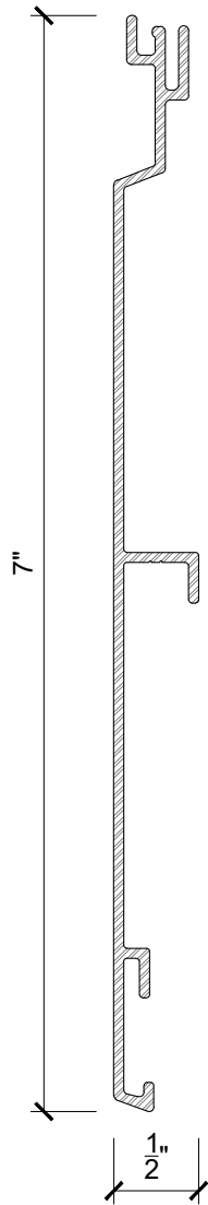
1 PV1 - PROFILE PV1-A SCALE 9"=1'-0"
