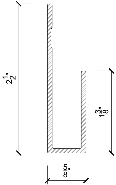
1 PL12 - PROFILE PL12-A SCALE 1'-0"=1'-0"
