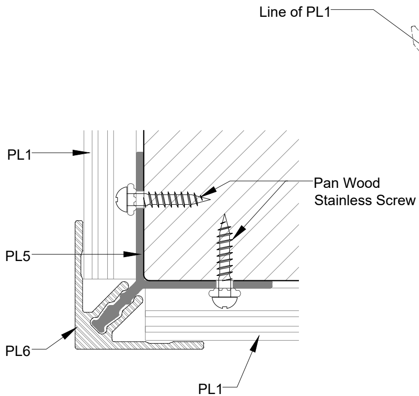
1 PL6 (TRIM) - APPLICATION PL6-B SCALE 1'-0"=1'-0"
