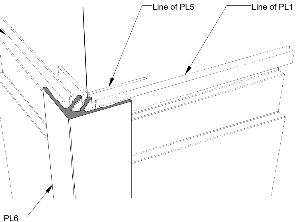
2 PL6 (TRIM) - APPLICATION - 3D VIEW PL6-B SCALE NTS
