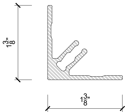
1 PL6 (TRIM) - PROFILE PL6-A SCALE 1'-0"=1'-0"
