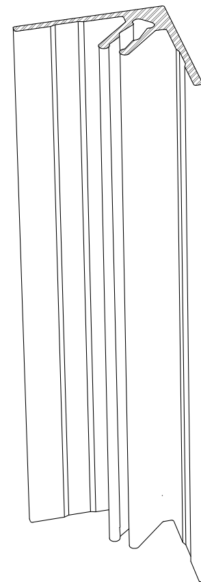
3 PL7 (RECEIVER) - 3D VIEW PL7-A SCALE NTS
