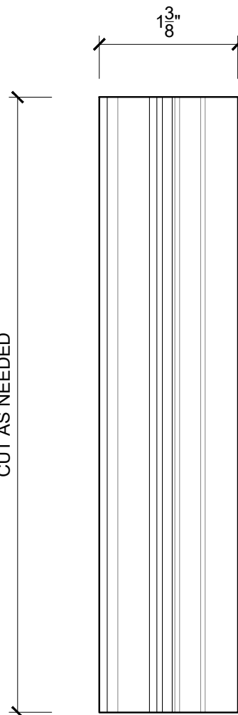
2 PL7 (RECEIVER) - FRONT PL7-A SCALE 9"=1'-0"
