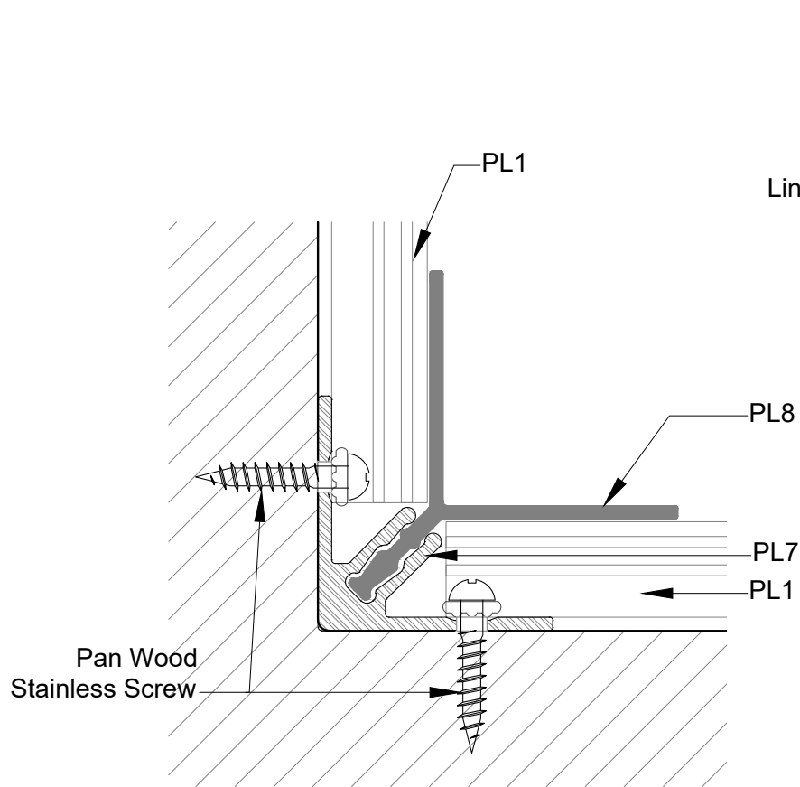
1 PL7 (RECEIVER) - APPLICATION PL7-B SCALE 1'-0"=1'-0"
