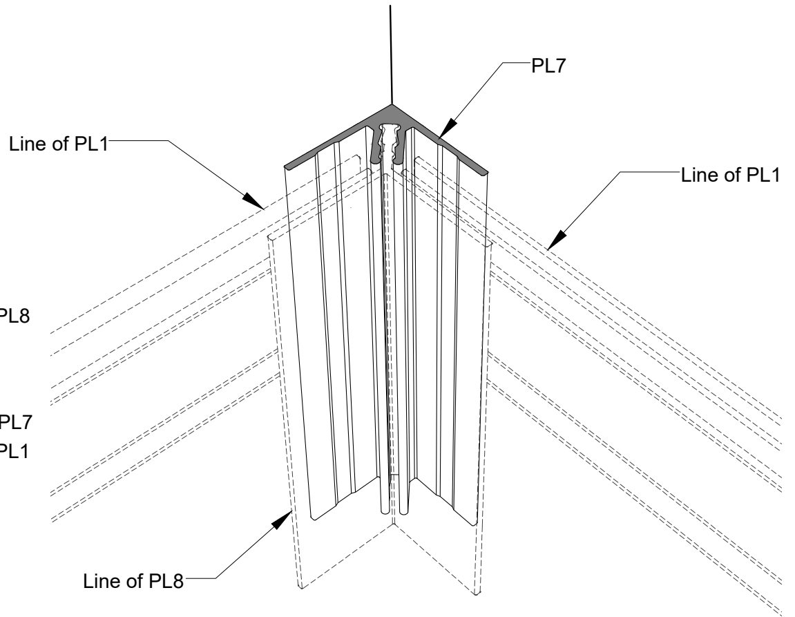
2 PL7 (RECEIVER) - APPLICATION - 3D VIEW PL7-B SCALE NTS
