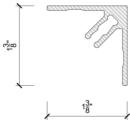
1 PL7 (RECEIVER) - PROFILE PL7-A SCALE 1'-0"=1'-0"
