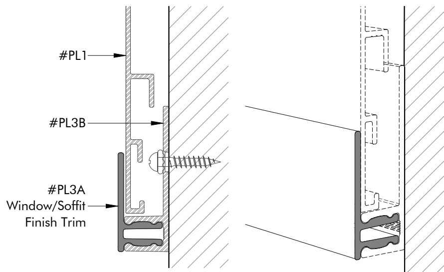
INSTALLATION VIEW (BOTTOM) Scale 9"=1'-0"
