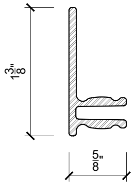
PROFILE VIEW Scale 1'-0"=1'-0"
