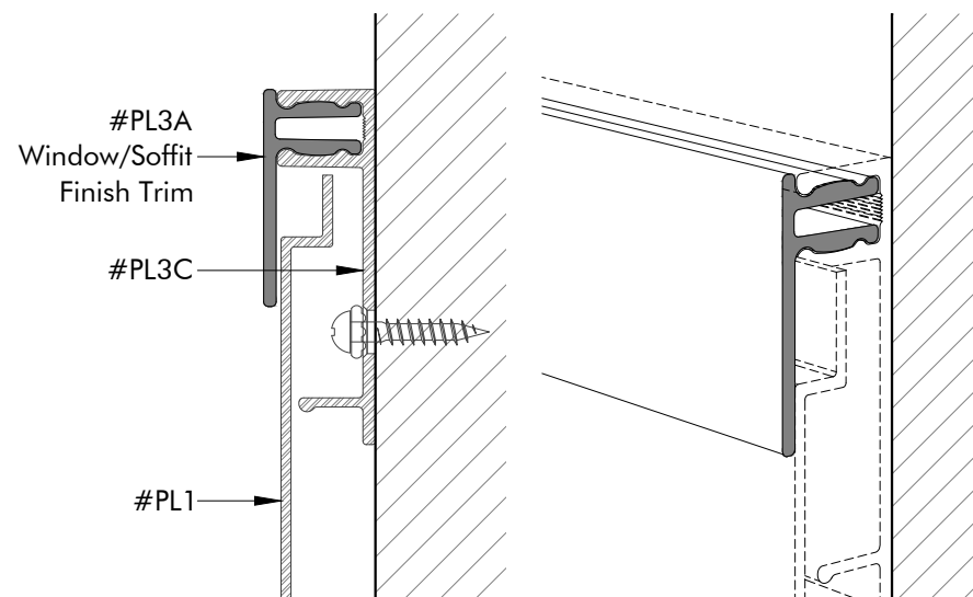
INSTALLATION VIEW (TOP) Scale 9"=1'-0"
