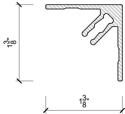
PROFILE VIEW Scale 1'-0"=1'-0"
