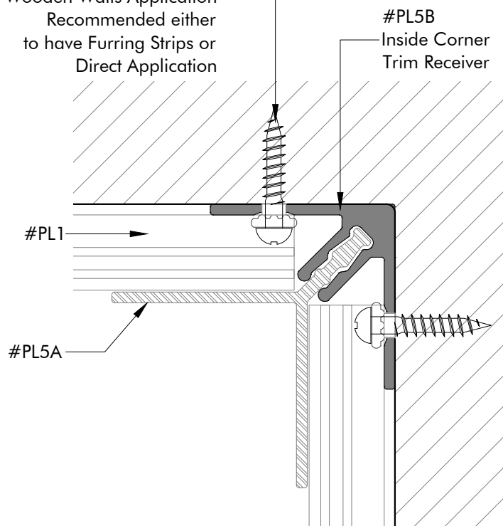
INSTALLATION VIEW Scale 1'-0"=1'-0"
