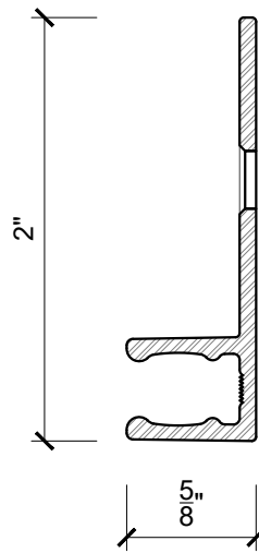
PROFILE VIEW Scale 1'-0"=1'-0"
