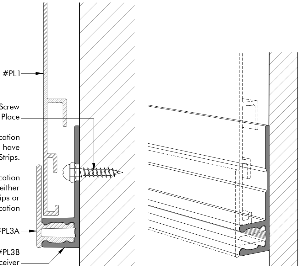
INSTALLATION VIEW Scale 1'-0"=1'-0"
