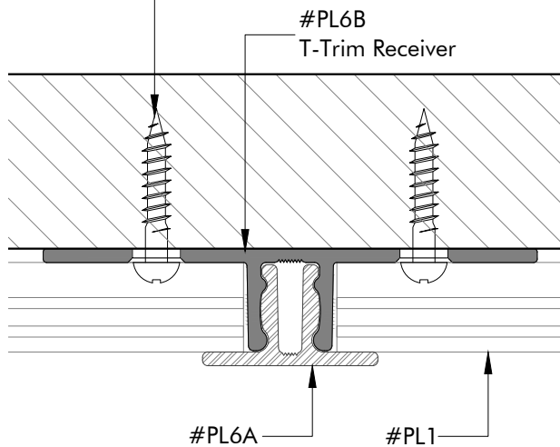
INSTALLATION VIEW Scale 1'-0"=1'-0"
