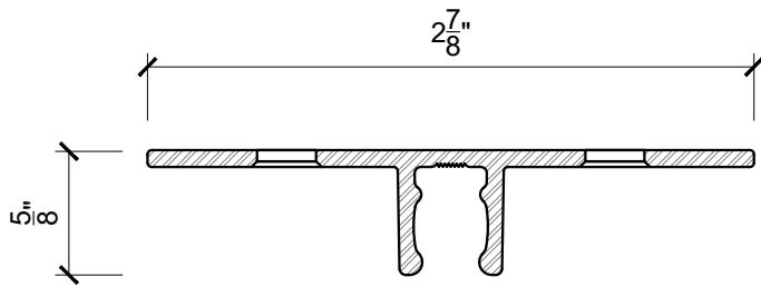
PROFILE VIEW Scale 1'-0"=1'-0"
