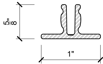
PROFILE VIEW Scale 1'-0"=1'-0"
