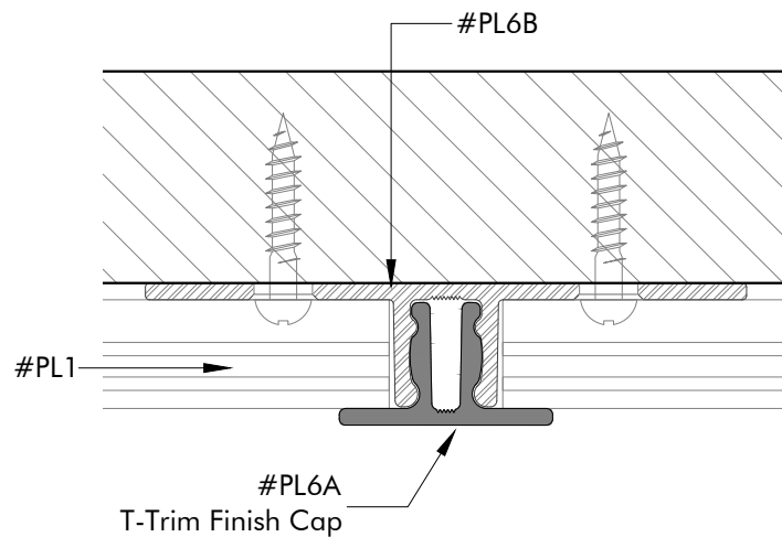
INSTALLATION VIEW Scale 1'-0"=1'-0"
