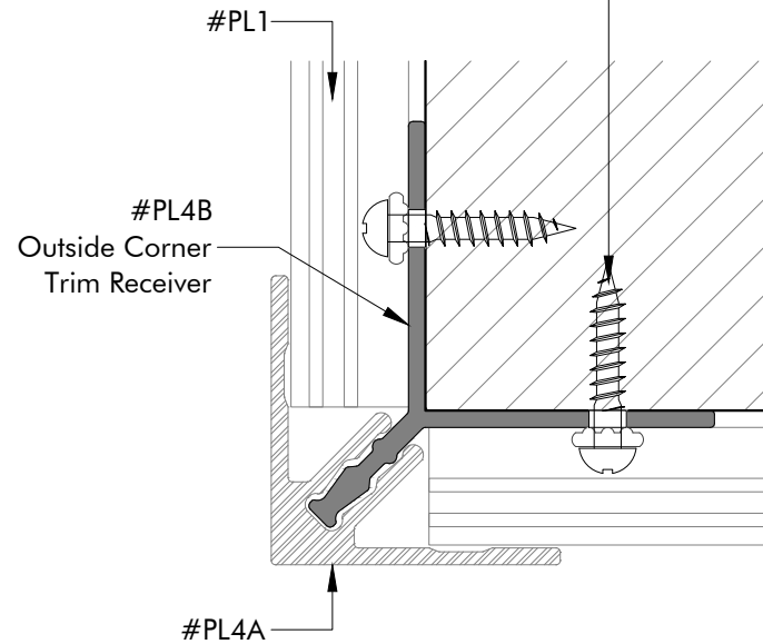
INSTALLATION VIEW Scale 1'-0"=1'-0"
