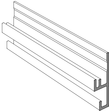
3D VIEW Scale NTS
