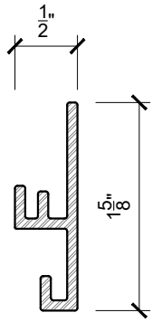
PROFILE VIEW Scale 6"=1'-0"
