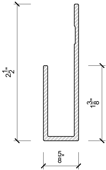
PROFILE VIEW Scale 1'-0"=1'-0"
